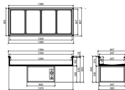
DCS 20D9934 (4斗) Ice bed (L)1394 x (W)607 x (H)560 Hole Size: (L)1380 x (W)593 mm
